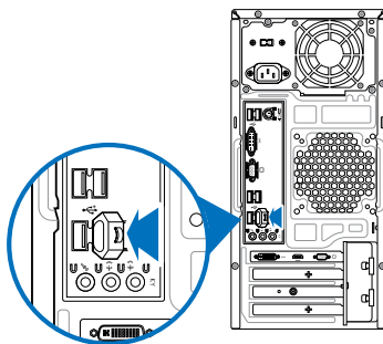
Painel traseiro
