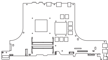
Motherboard with ports and connectors
