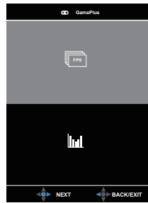
GamePlus-FPS Counter
