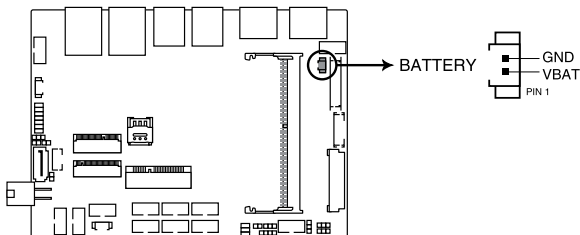
Battery connector
