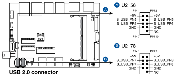
USB 2.0 connector
