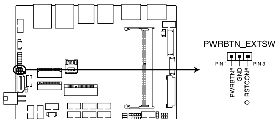
Power button connector
