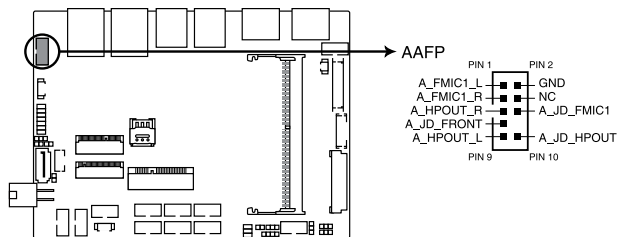
Line_out/Mic connector
