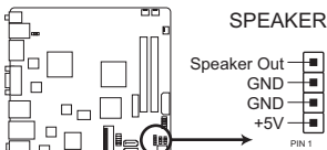
AT5IONT-I DELUXE Speaker out connector
