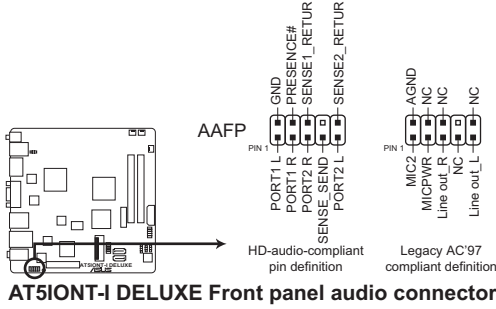
AT5IONT-I DELUXE Front panel audio connector
