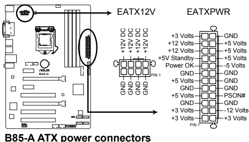
B85-A ATX power connectors
