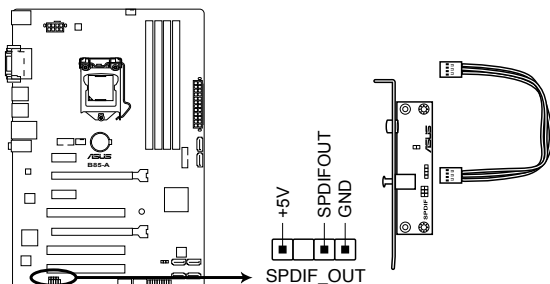
B85-A Digital audio connector
