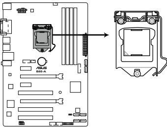
B85-A CPU socket LGA1150
