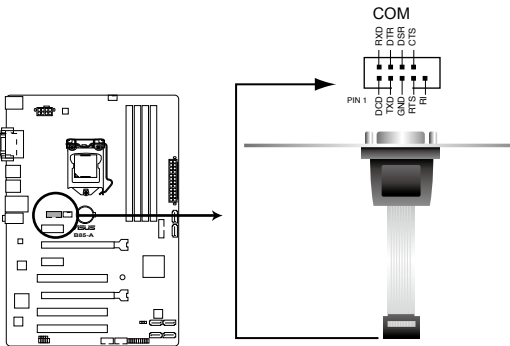
B85-A Serial port (COM) connector
