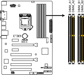
B85-A 240-pin DDR3 DIMM sockets
