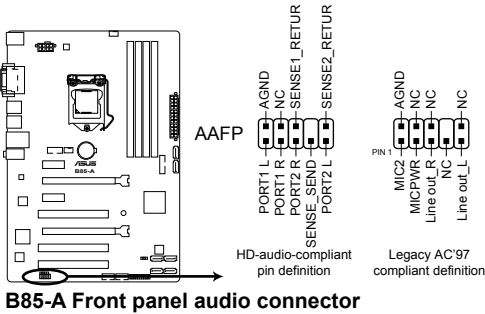
B85-A Front panel audio connector
