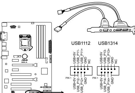
B85-A USB2.0 connectors
