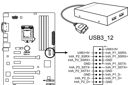
B85-A USB3.0 Front panel connector
