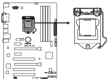
B85-PLUS CPU socket LGA1150
