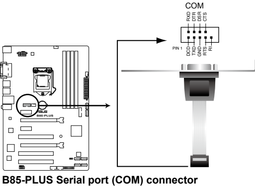
B85-PLUS Serial port (COM) connector
