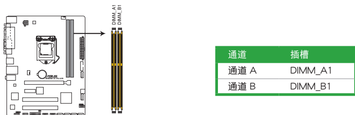
B85M-D PLUS 240-pin DDR3 DIMM sockets
