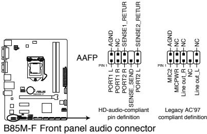
B85M-F Front panel audio connector
