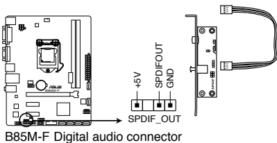
B85M-F Digital audio connector
