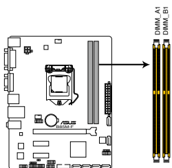
B85M-F 240-pin DDR3 DIMM sockets
