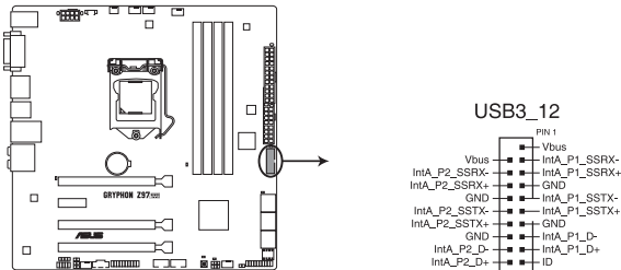
GRYPHON Z97 ARMOR EDITION USB3.0 connector
