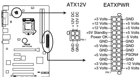
H81-PLUS ATX power connectors
