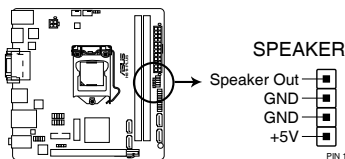
H81I-PLUS Speaker Out Connector
