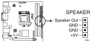
H81I-PLUS Speaker Out Connector
