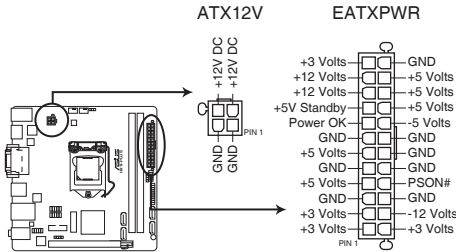
H81I-PLUS ATX power connectors
