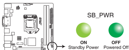
H81I-PLUS Onboard LED
