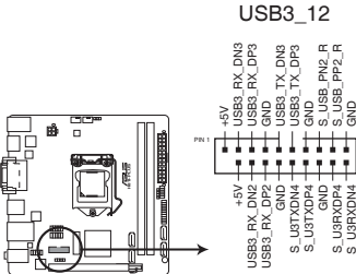
H81-PLUS USB3.0 Front panel connector
