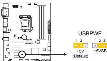
H87M-E USB device wake up
