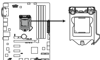
H87M-E CPU socket LGA1150
