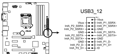
H87M-PRO USB3.0 Front panel connector
