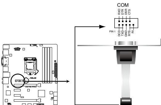
H87M-PRO Serial port (COM) connector
