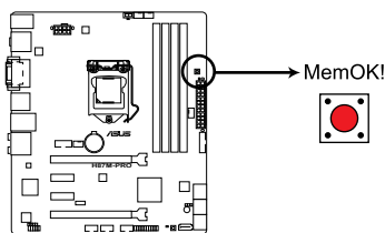
H87M-PRO MemOK! switch
