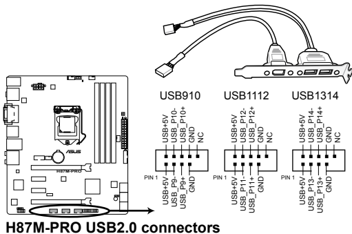
H87M-PRO USB2.0 connectors
