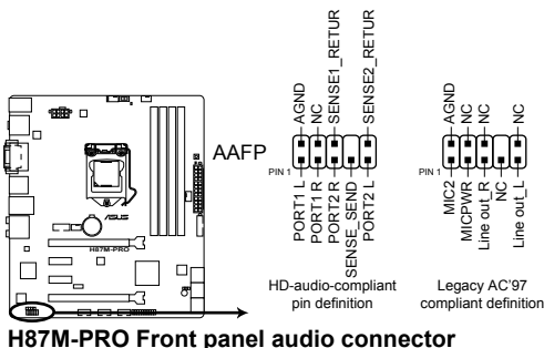
H87M-PRO Front panel audio connector
