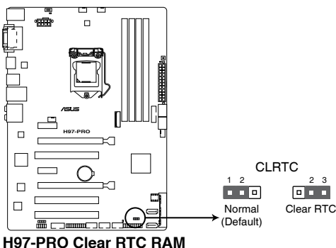
H97-PRO Clear RTC RAM
