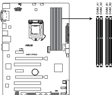
H97-PRO 240-pin DDR3 DIMM sockets
