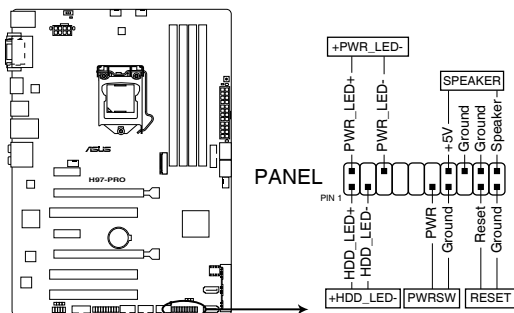
H97-PRO System panel connector
