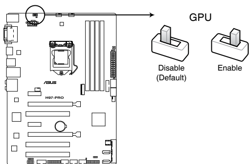
H97-PRO GPU Boost switch
