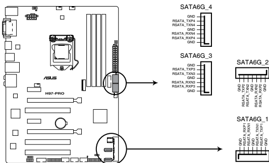
H97-PRO Intel® SATA 6.0Gb/s connectors
