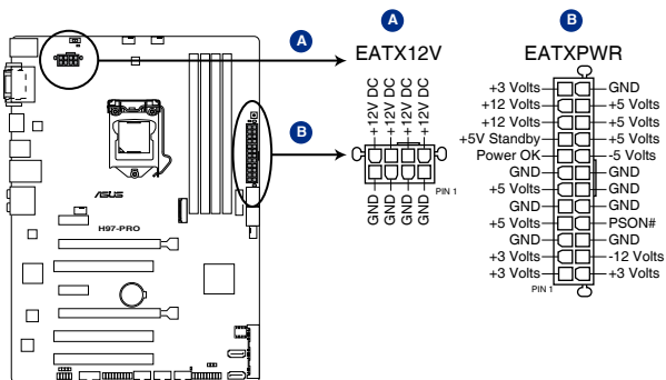
H97-PRO ATX power connectors
