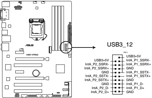
H97-PRO USB3.0 connector
