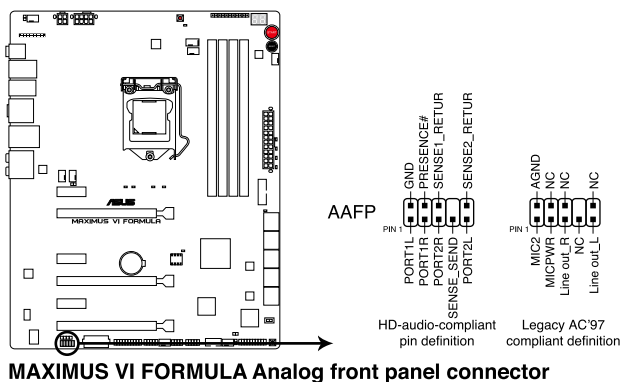
MAXIMUS VI FORMULA Analog front panel connector
