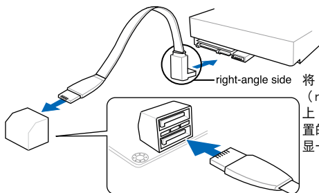
MAXIMUS VI FORMULA Intel® SATA 6 Gb/s connectors
