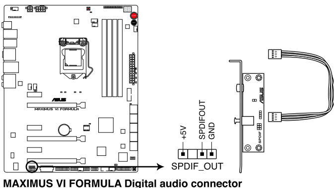
MAXIMUS VI FORMULA Digital audio connector
