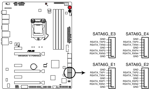
MAXIMUS VI FORMULA ASMedia® SATA 6 Gb/s connectors
