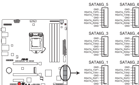
MAXIMUS VII GENE Intel® SATA 6 Gb/s connectors
