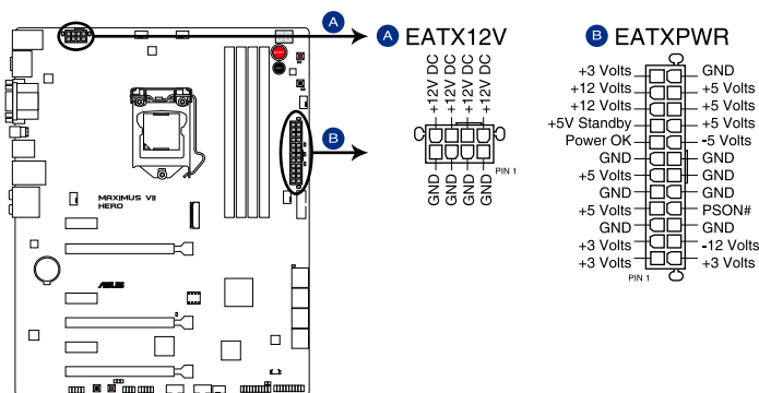
MAXIMUS VII HERO ATX power connectors
