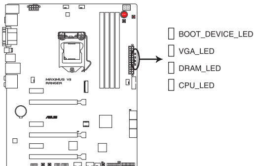
MAXIMUS VII RANGER CPU/ DRAM/ VGA/ BOOT_DEVICE LED
