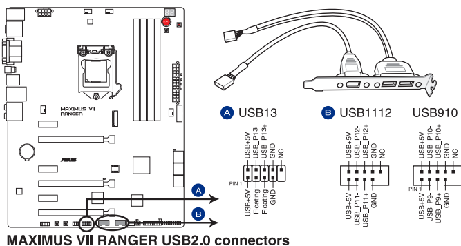
MAXIMUS VII RANGER USB2.0 connectors
