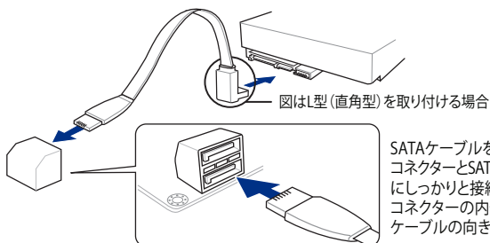
MAXIMUS VII RANGER Intel® SATA 6 Gb/s connectors
