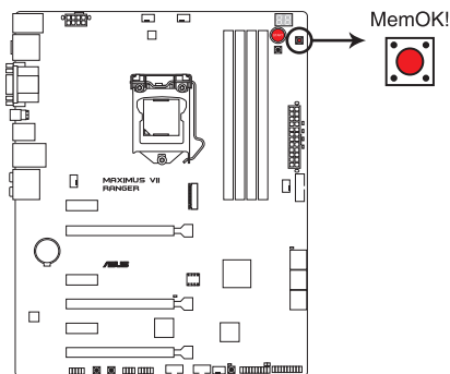
MAXIMUS VII RANGER MemOK! button
