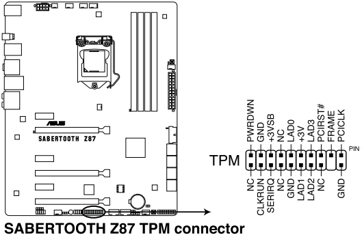
SABERTOOTH Z87 TPM connector
