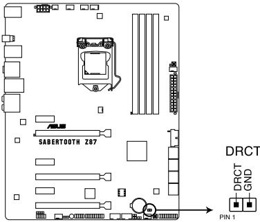
SABERTOOTH Z87 DirectKey connector
