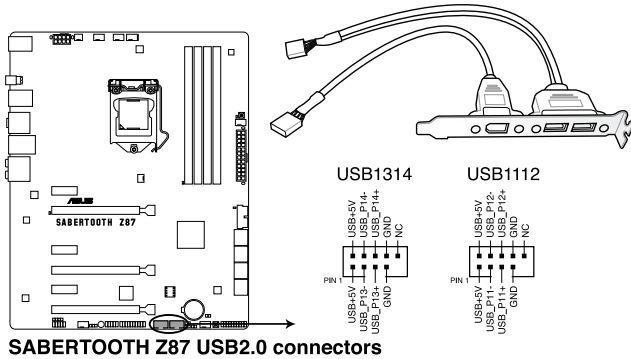
SABERTOOTH Z87 USB2.0 connectors
