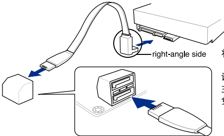
SABERTOOTH Z97 MARK 1 Intel® SATA 6 Gb/s connectors
