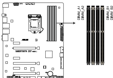
SABERTOOTH Z97 MARK 1 240-pin DDR3 DIMM socket
