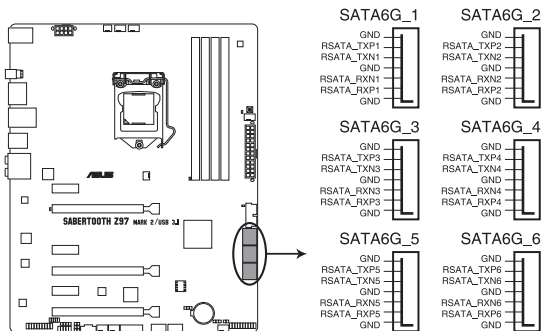
SABERTOOTH Z97 MARK 2/USB 3.1 Intel® SATA 6 Gb/s connectors
