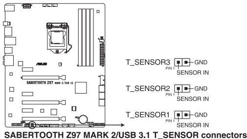
SABERTOOTH Z97 MARK 2/USB 3.1 T_SENSOR connectors
