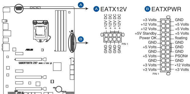
SABERTOOTH Z97 MARK 2/USB 3.1 ATX power connectors
