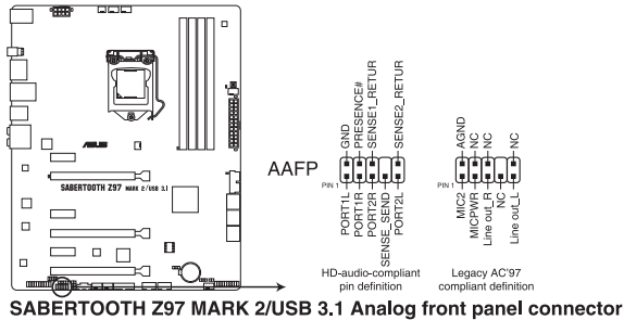
SABERTOOTH Z97 MARK 2/USB 3.1 Analog front panel connector
