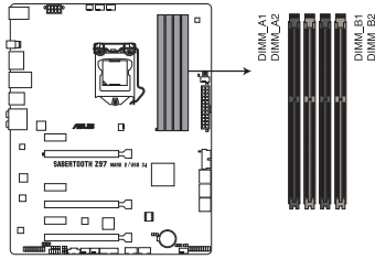
SABERTOOTH Z97 MARK 2/USB 3.1 240-pin DDR3 DIMM socket
