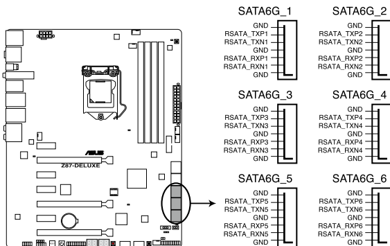
Z87-DELUXE Intel® SATA 6.0 Gb/s connectors
