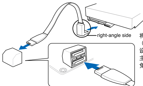
Z87-DELUXE Intel® SATA 6.0 Gb/s connectors
