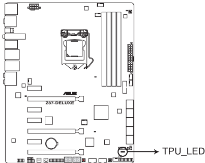
LED TPU de la Z87-DELUXE
