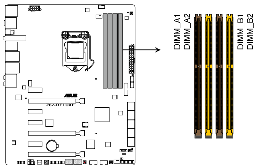
Z87-DELUXE 240-pin DDR3 DIMM socket
