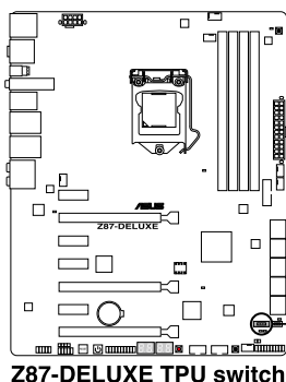
Z87-DELUXE TPU switch
