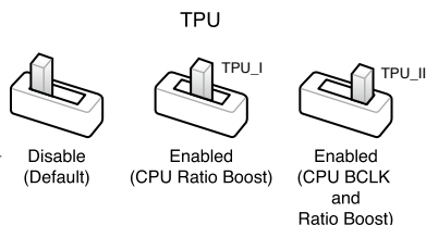
Z87-DELUXE TPU switch
