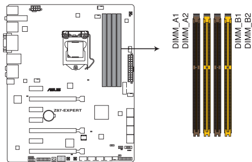
Z87-EXPERT 240-pin DDR3 DIMM socket
