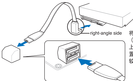
Z87-EXPERT Intel® SATA 6.0 Gb/s connectors
