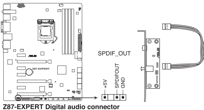
Z87-EXPERT Digital audio connector
