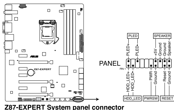
Z87-EXPERT System panel connector
