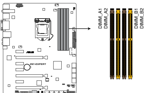
Z87-EXPERT 240-pin DDR3 DIMM slots
