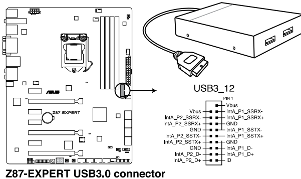
Z87-EXPERT USB3.0 connector
