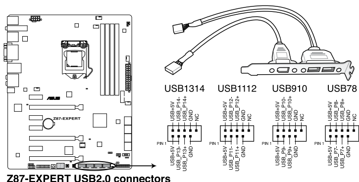
Z87-EXPERT USB2.0 connectors
