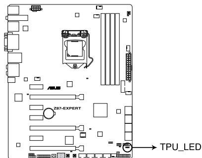
Z87-EXPERT TPU LEDs
