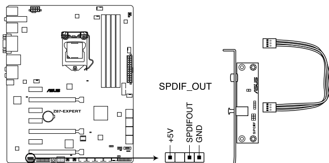
Z87-EXPERT Digital audio connector
