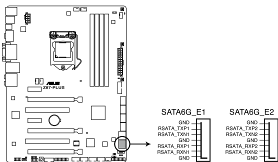
Z87-PLUS ASMedia® SATA 6.0 Gb/s connectors
