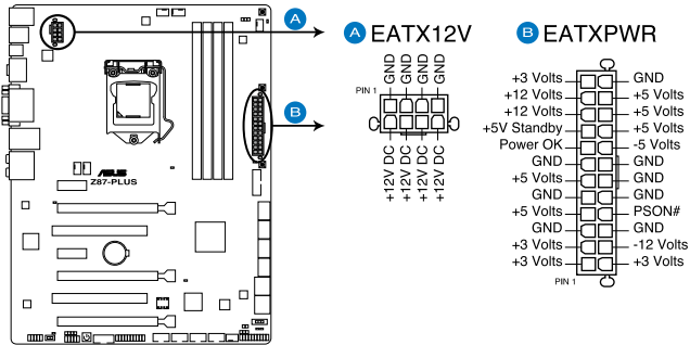
Z87-PLUS ATX power connectors
