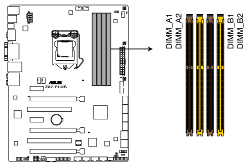
Z87-PLUS 240-pin DDR3 DIMM socket
