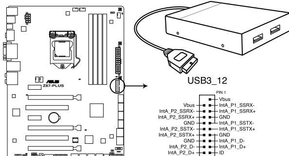
Z87-PLUS USB3.0 connector
