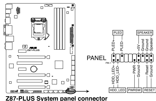
Z87-PLUS System panel connector
