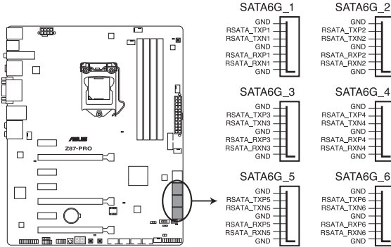
Z87-PRO Intel® SATA 6.0 Gb/s connectors
