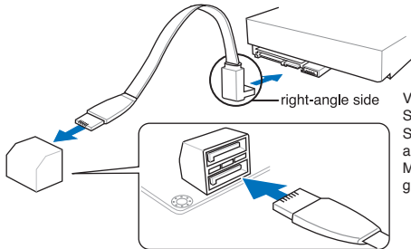
Z87-PRO Intel® SATA 6.0 Gb/s connectors
