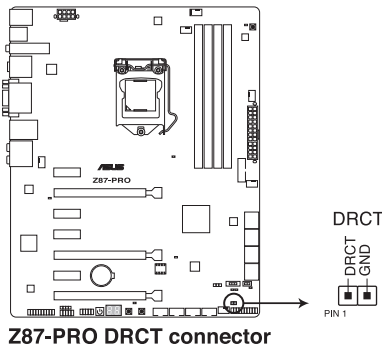
Z87-PRO DRCT connector
