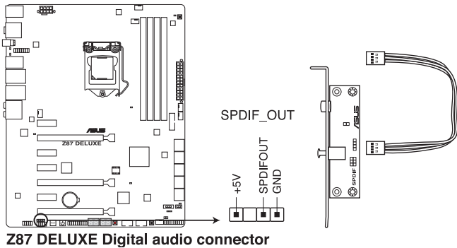
Z87 DELUXE Digital audio connector
