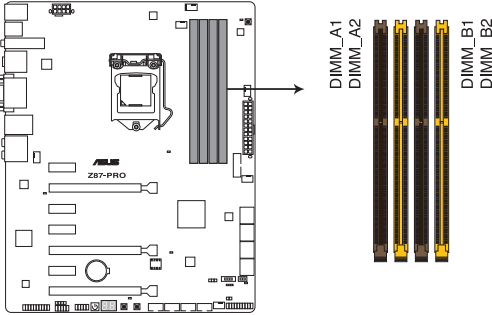
Z87-PRO 240-pin DDR3 DIMM socket
