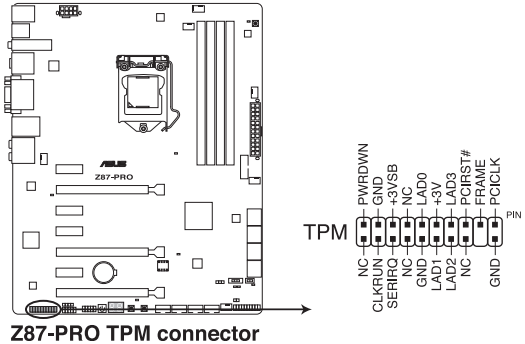
Z87-PRO TPM connector
