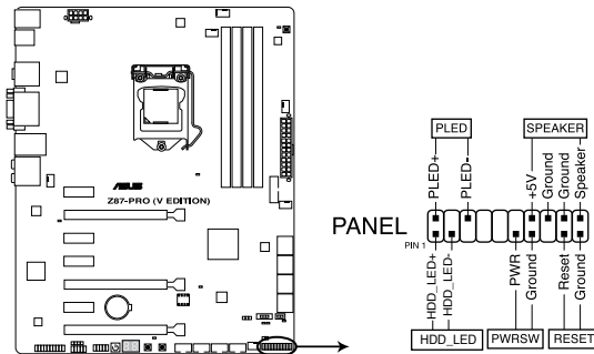
Z87-PRO (V EDITION) System panel connector
