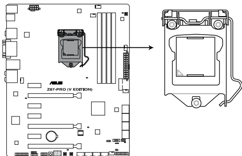
Z87-PRO (V EDITION) CPU LGA1150
