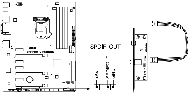
Z87-PRO (V EDITION) Digital audio connector
