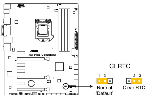
Z87-PRO (V EDITION) Clear RTC RAM
