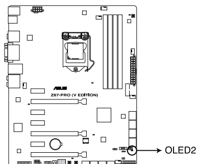
Z87-PRO (V EDITION) EPU LED
