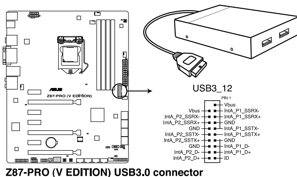
Z87-PRO (V EDITION) USB3.0 connector
