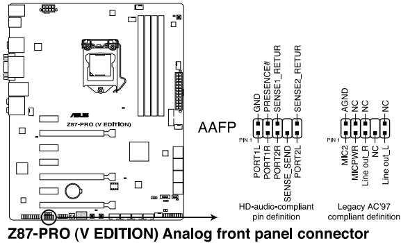
Z87-PRO (V EDITION) Analog front panel connector
