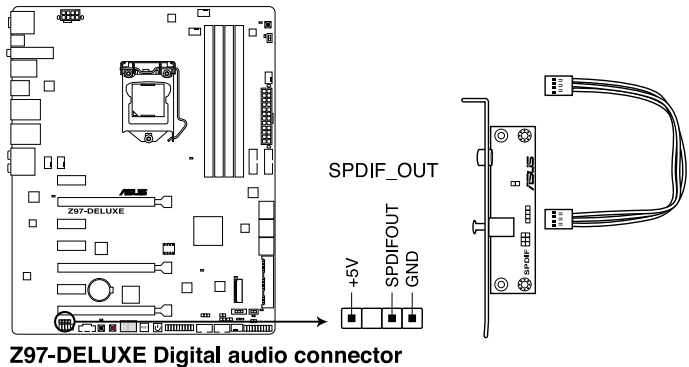
Z97-DELUXE Digital audio connector
