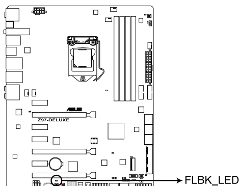
Z97-DELUXE FLBK_LED
