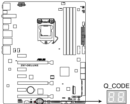
Z97-DELUXE Q-Code LED
