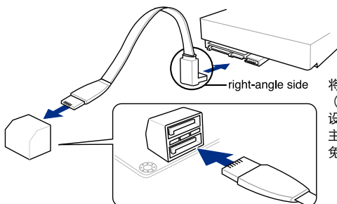
Z97-DELUXE Intel® SATA 6 Gb/s connectors
