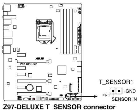
Z97-DELUXE T_SENSOR connector
