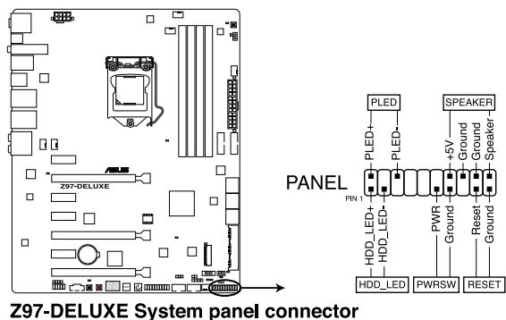
Z97-DELUXE System panel connector
