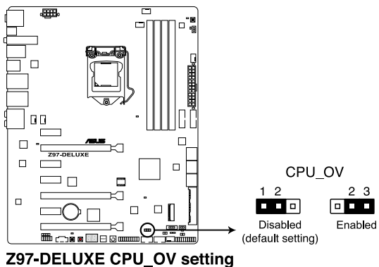
Z97-DELUXE CPU_OV setting
