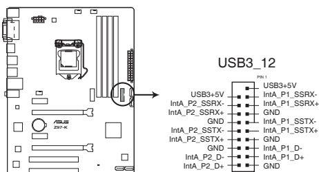
Z97-K USB3.0 front panel connector
