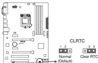
Z97-K Clear RTC RAM
