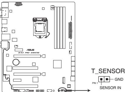
B150 PRO GAMING T_SENSOR connector
