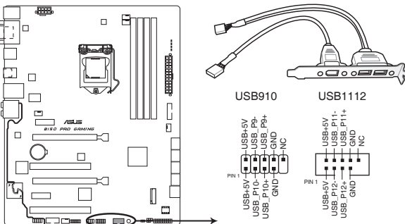
B150 PRO GAMING USB2.0 connectors
