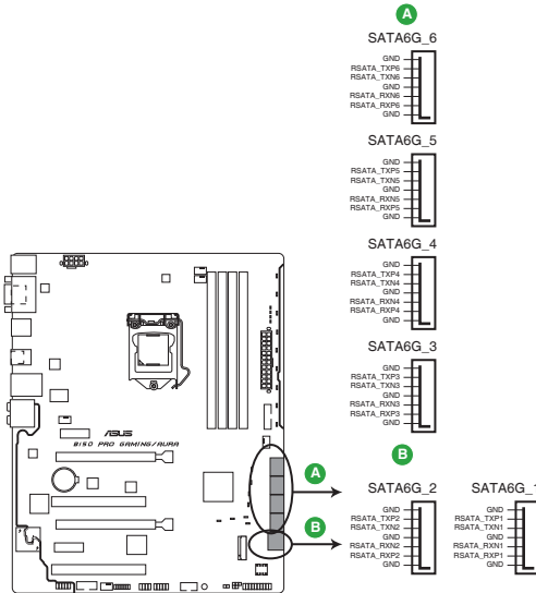
B150 PRO GAMING/AURA Intel® SATA 6.0Gb/s connectors
