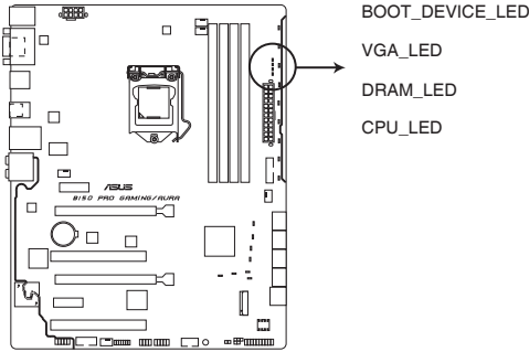
B150 PRO GAMING/AURA CPU/DRAM/ BOOT_DEVICE/VGA LED
