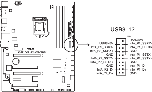
B150 PRO GAMING/AURA USB3.0 Front panel connector
