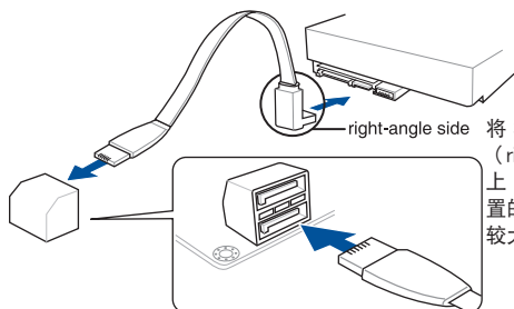
MAXIMUS VIII EXTREME Intel® SATA 6 Gb/s connectors
