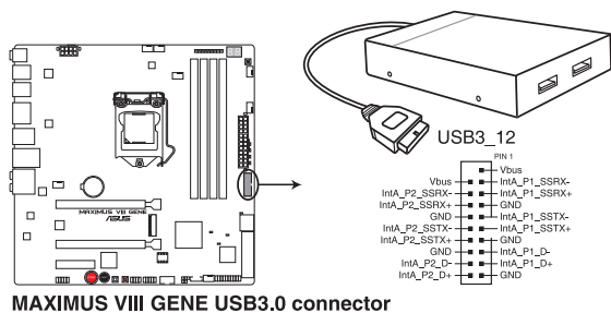
MAXIMUS VIII GENE USB3.0 connector
