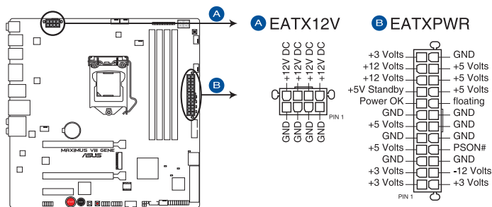
MAXIMUS VIII GENE ATX power connectors
