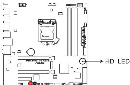
MAXIMUS VIII GENE Hard Disk LED
