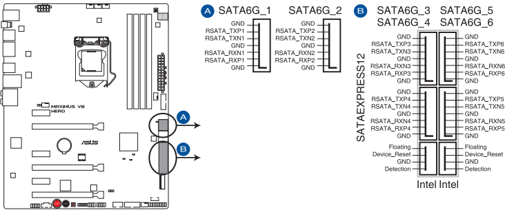
MAXIMUS VIII HERO Intel® SATA 6 Gb/s connectors
