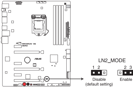
MAXIMUS VIII HERO LN2_MODE setting
