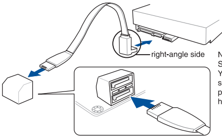
MAXIMUS VIII HERO Intel® SATA 6 Gb/s connectors
