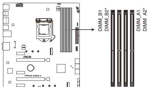
PRIME Z390-A 288-pin DDR4 DIMM socket
