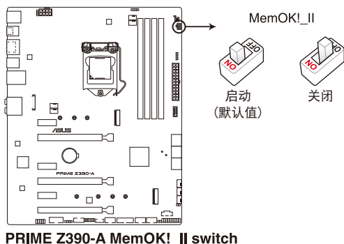
PRIME Z390-A MemOK!_II switch
