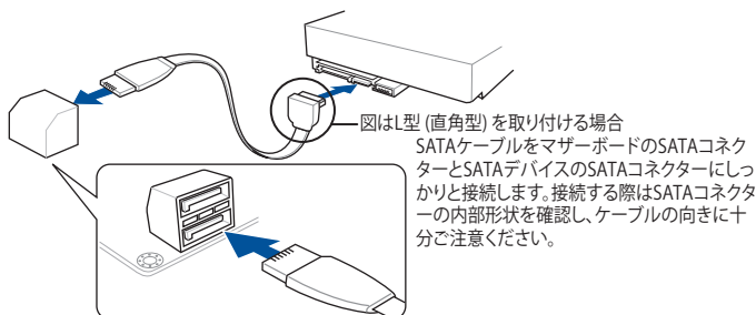
PRIME Z390-A Intel® Serial ATA 6 Gb/s connectors
