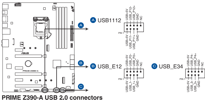
PRIME Z390-A USB 2.0 connectors
