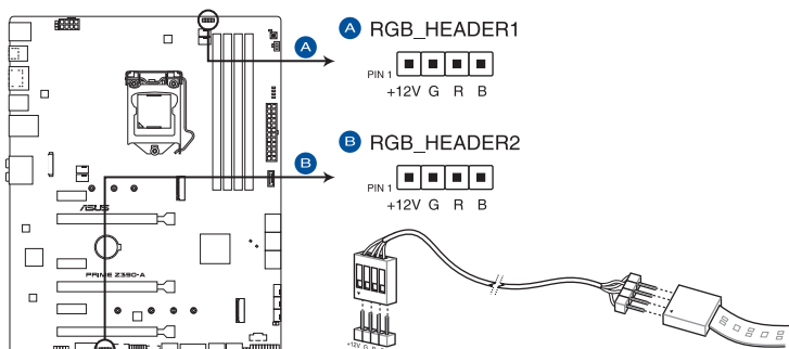
PRIME Z390-A RGB_HEADER connectors
