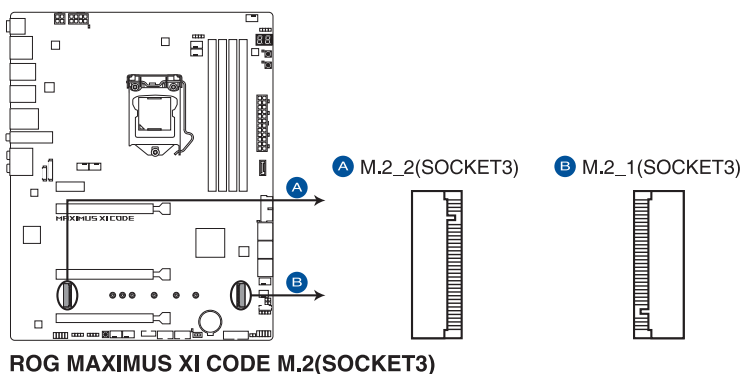
ROG MAXIMUS XI CODE M.2(SOCKET3)
