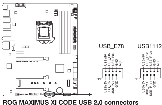
ROG MAXIMUS XI CODE USB 2.0 connectors
