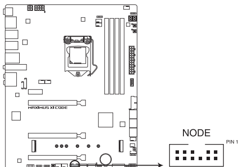
ROG MAXIMUS XI CODE NODE
