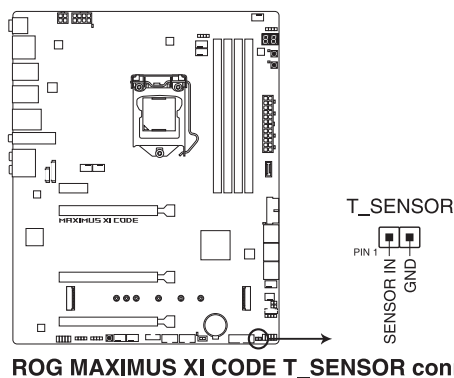
ROG MAXIMUS XI CODE T_SENSOR connector
