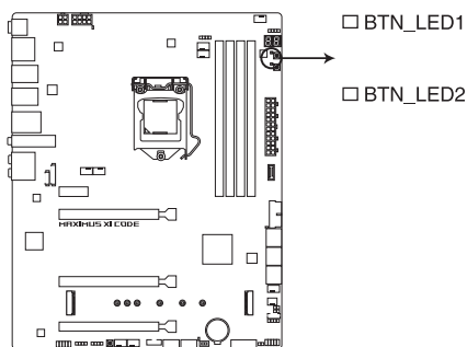
ROG MAXIMUS XI CODE BTN_LED
