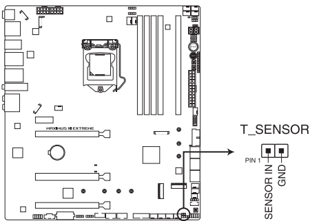
ROG MAXIMUS XI EXTREME Thermal sensor connector
