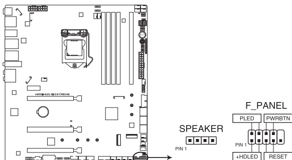
ROG MAXIMUS XI EXTREME System panel connector
