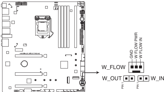
ROG MAXIMUS XI EXTREME W_IN, W_OUT & W_Flow
