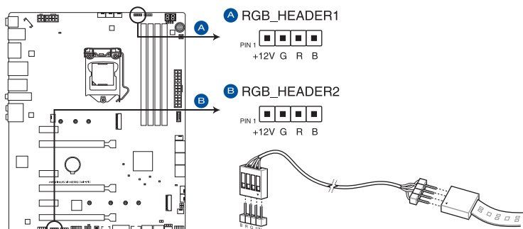
ROG MAXIMUS XI HERO (WI-FI) RGB_HEADER connectors
