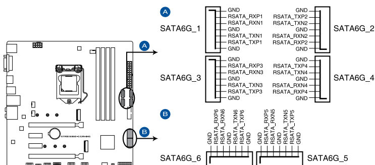
ROG STRIX B360-G GAMING Intel® Serial ATA 6 Gb/s connectors
