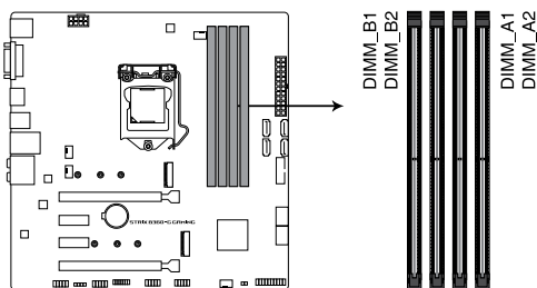
ROG STRIX B360-G GAMING 288-pin DDR4 DIMM socket
