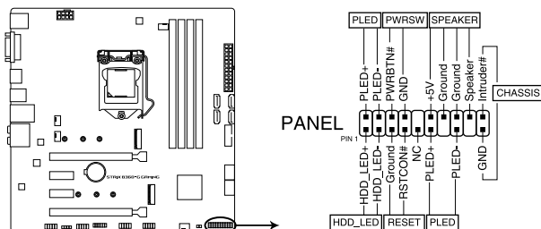
ROG STRIX B360-G GAMING System panel connector
