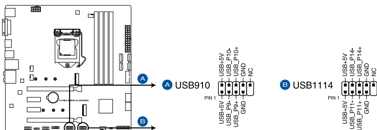
ROG STRIX B360-G GAMING USB 2.0 connectors
