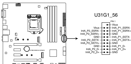
ROG STRIX B360-G GAMING USB 3.1 Gen 1 connector
