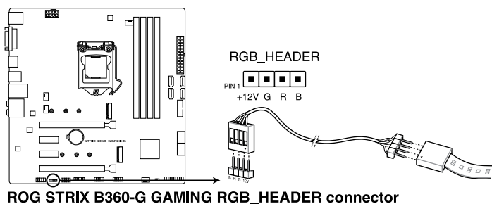
ROG STRIX B360-G GAMING RGB_HEADER connector
