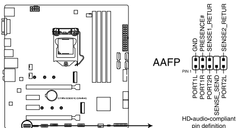
ROG STRIX B360-G GAMING Front panel audio connector
