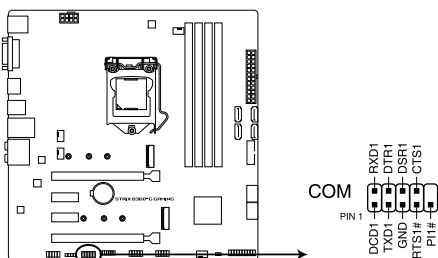
ROG STRIX B360-G GAMING Serial port connector
