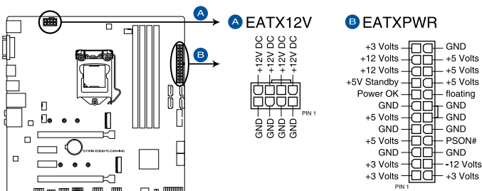
ROG STRIX B360-G GAMING ATX power connectors
