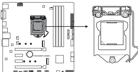
ROG STRIX B360-G GAMING CPU LGA1151
