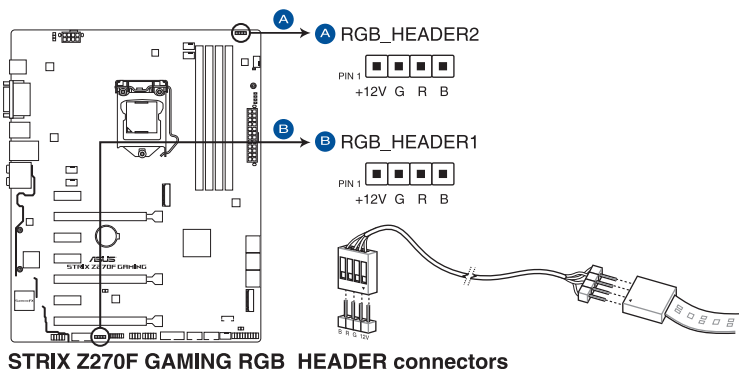
STRIX Z270F GAMING RGB_HEADER connectors
