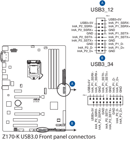
Z170-K USB3.0 Front panel connectors
